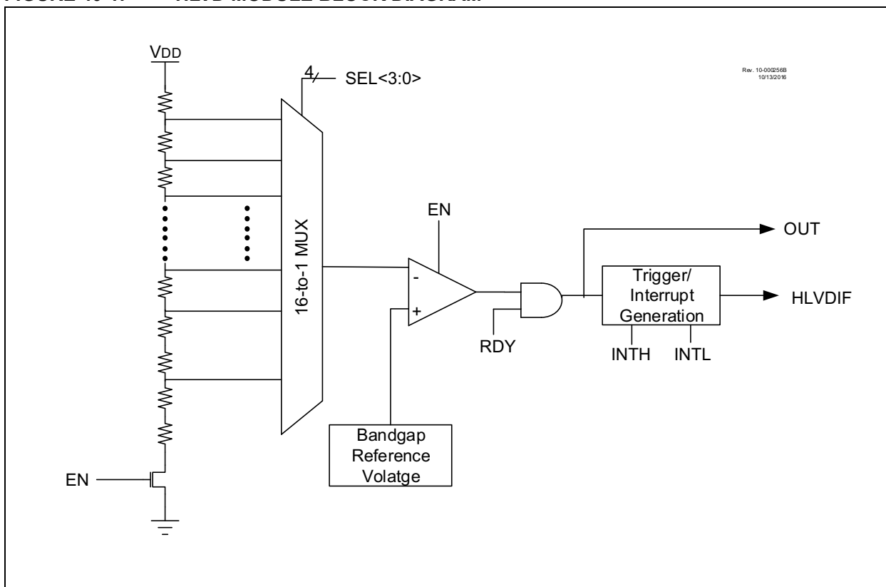
FIGURE 40-1: HLVD MODULE BLOCK DIAGRAM
